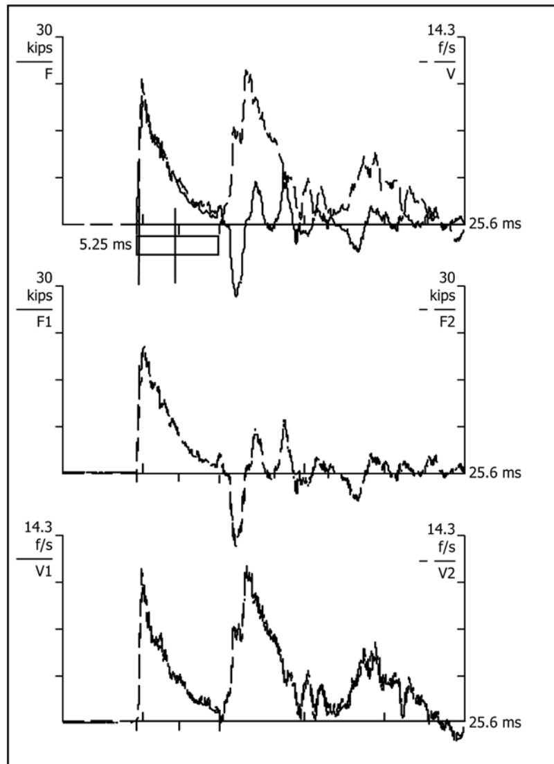
NOTE 1—1 kip = 1000 lbf = 4.448 kN and 14.3 ft/s = 4.36 m/s. FIG. 1 Example Force- and Velocity-Time Measurement for SPT
