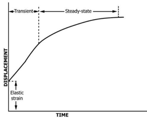
FIG. 5 Typical Creep Curve
