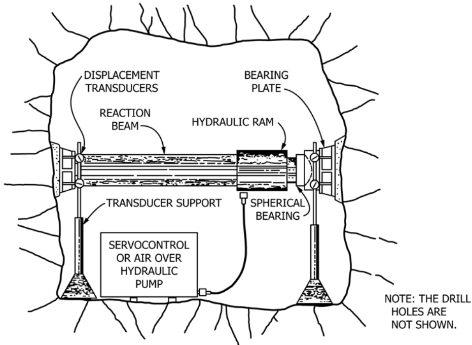
FIG. 3 Typical Rigid Plate Bearing Test Setup Schematic
