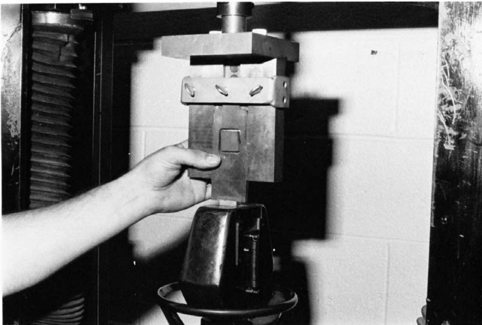
FIG. 5 Specimen Loaded in Shearing Fixture
