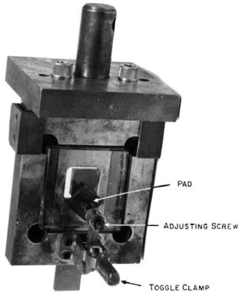
FIG. 6 Rear View of Fixture with Specimen Clamped in Place
