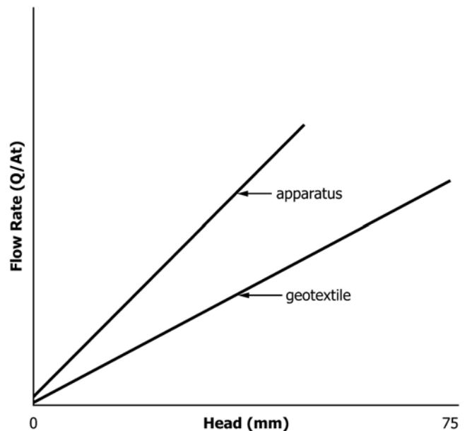
FIG. 3 Calibration Curve
