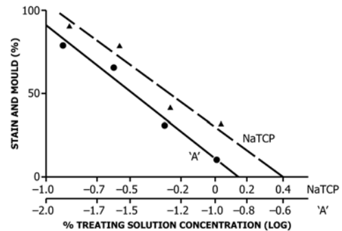
FIG. 4 Example of CGo Determination for Unknown Chemical A, Compared with Sodium Tetrachlorophenate (NaTCP)
