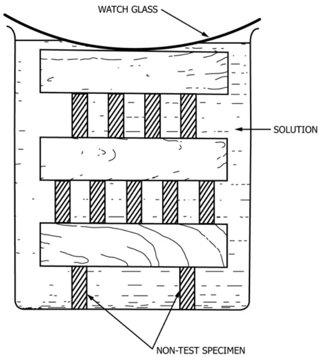
FIG. 3 Arrangement of Test Material for Treatment in a 600-mL Beaker
