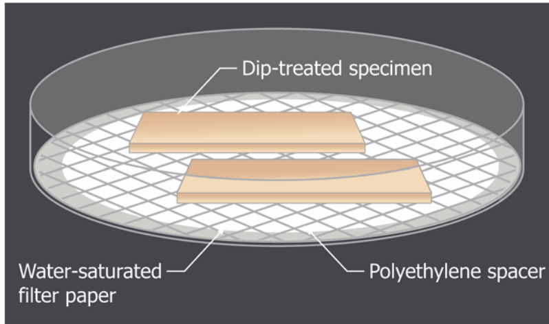
FIG. 2 Arrangement of Treated Wood Specimens on Polyethylene Spacing Within the Petri Dishes Before Incubation
