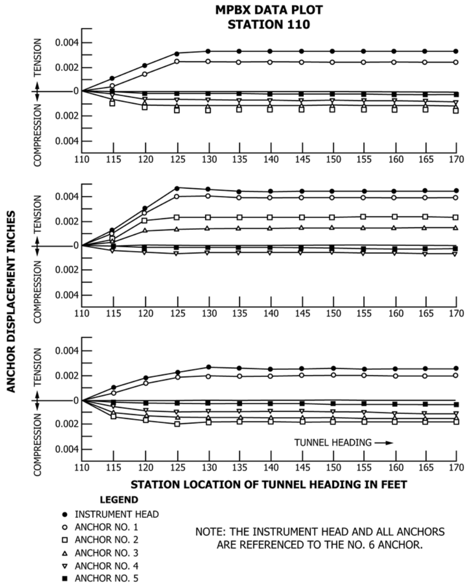
FIG. 13 Hypothetical Extensometer Data Plot
