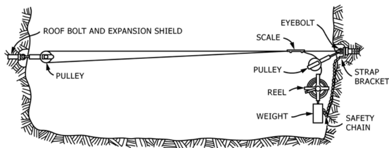
FIG. 3 Tape Extensometer with Vernier Readout and Deadweight
