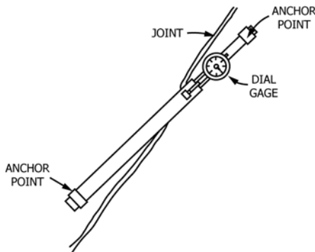
FIG. 5 Joint Meters
