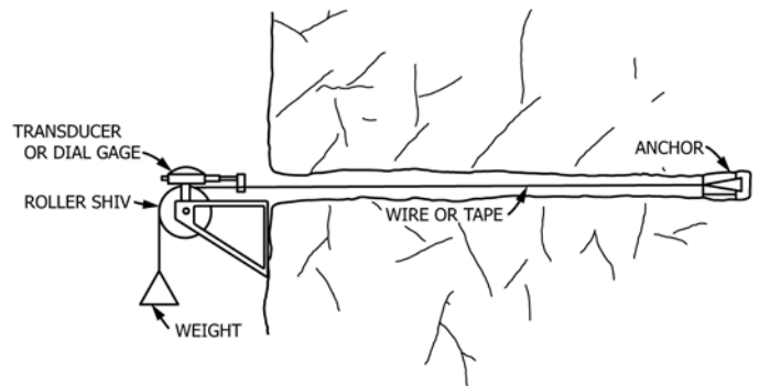
FIG. 6 Wire Extensometers
