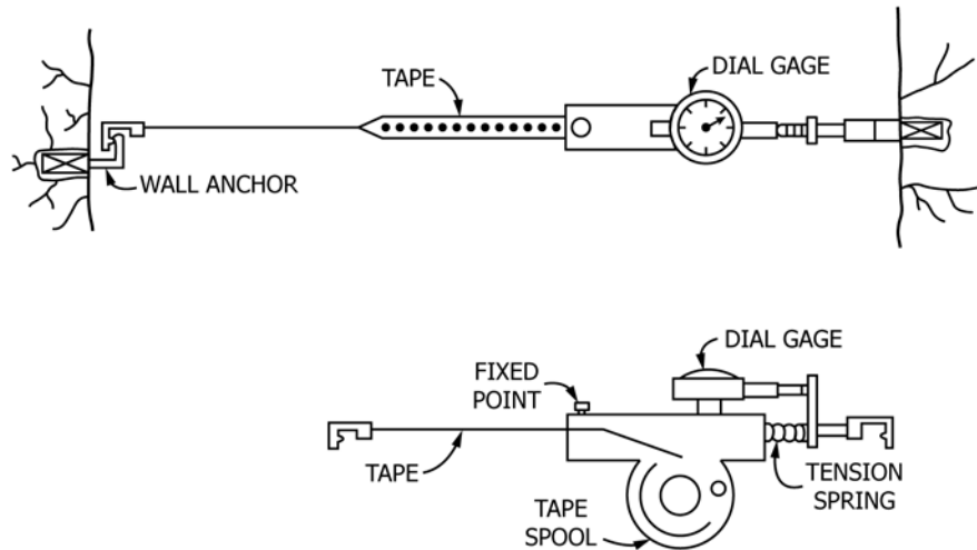
FIG. 4 Tape Extensometer with Dial Gage and Tension Spring
