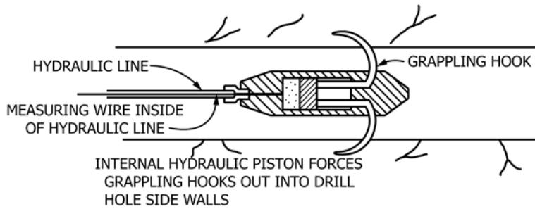
FIG. 9 Hydraulic Anchors
