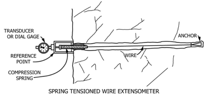
SPRING TENSIONED WIRE EXTENSOMETER
