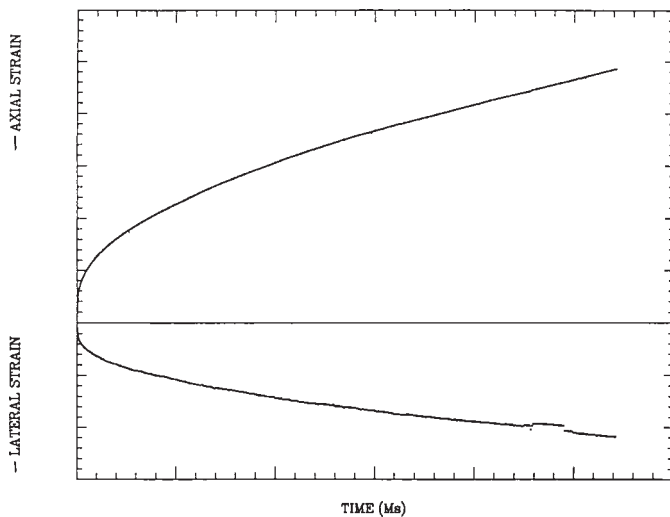
FIG. 1 Typical Strain-Versus-Time Curves
