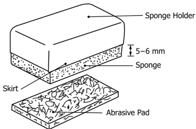
FIG. 2 Abrasion Boat Components
