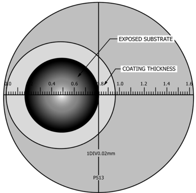
FIG. 7 Typical View Through Microscope of Cutter/Drill Cut
