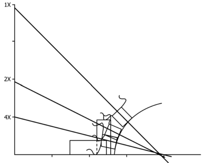
FIG. 5 Rotary Tool Block—Positions for Various Cutting Angles (Slopes)
