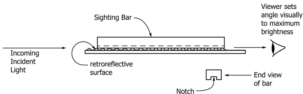
FIG. 7 Example of Alignment to 90° Entrance Angle with a Visual Sighting Bar
