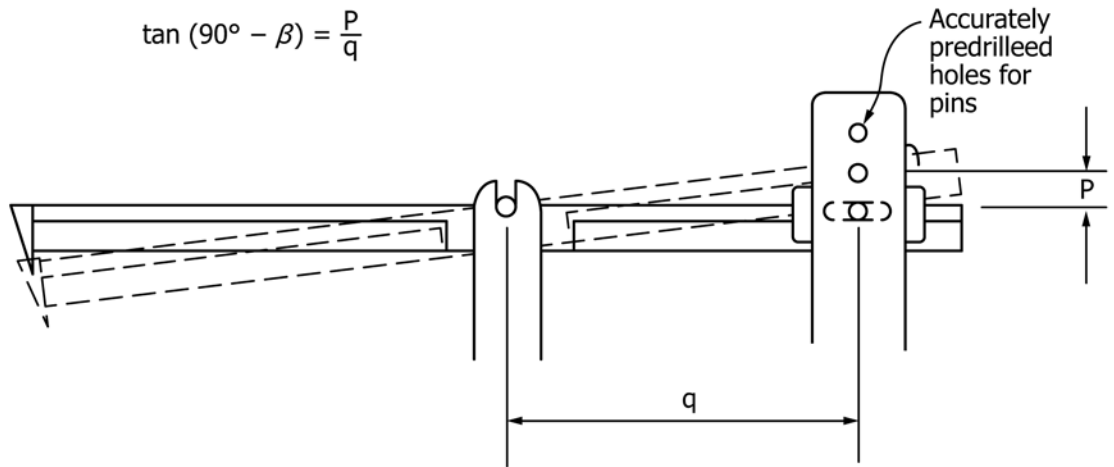
FIG. 6 Example of Alignment Procedure for Specimen Holder with Fixed Entrance Angle Setting
