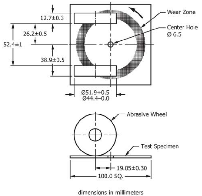
This schematic shows the proper wheel position in relation to the turntable platform.
