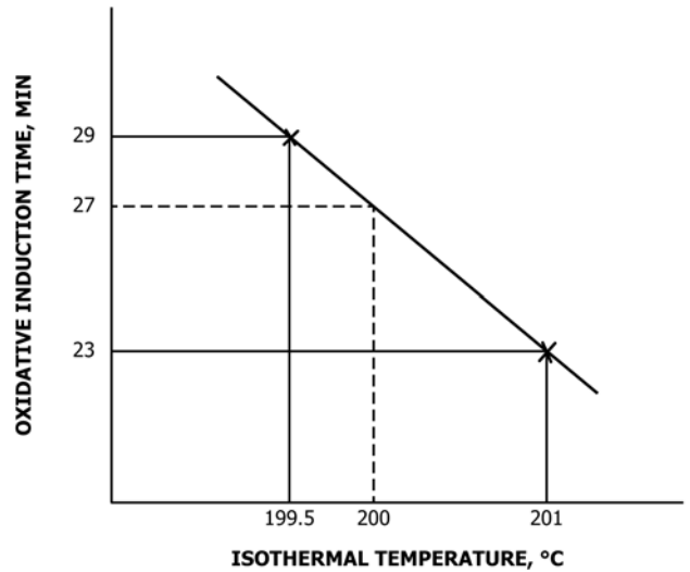
FIG. A1.1 Example of the Linear-Interpolation Technique Used to Estimate the OIT at 200.0^\circ\text{C}
