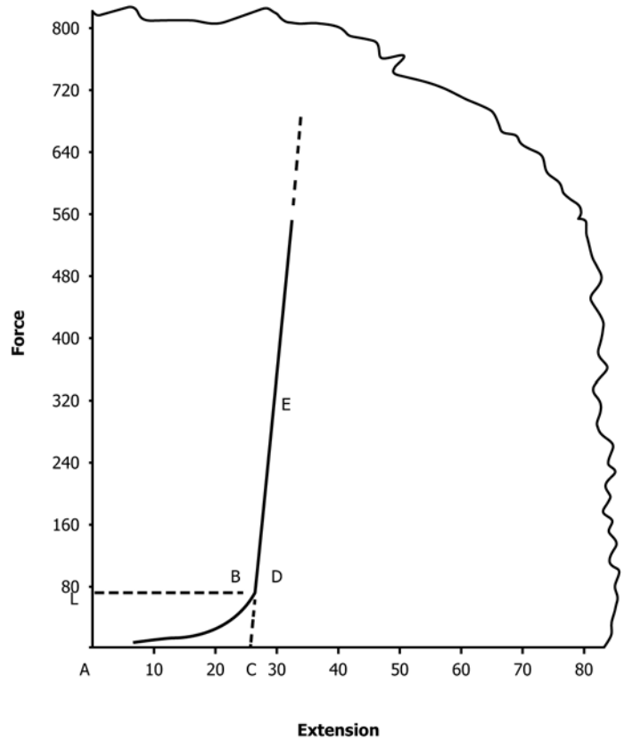
FIG. 1 Example Chart For Determining of Tensile Force Using Option C
