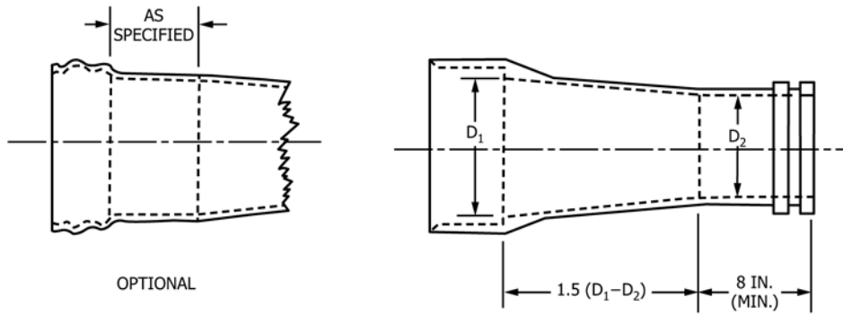
FIG. 1 Concentric Reducer
