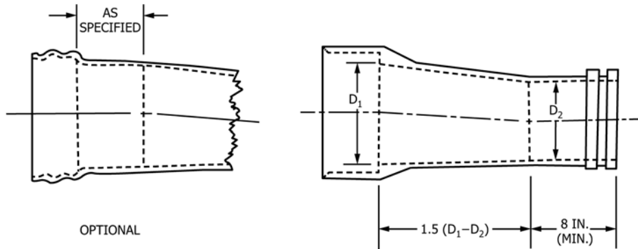
FIG. 2 Eccentric Reducer
