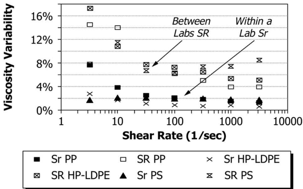
NOTE 1—By material, within-laboratory and laboratory-to-laboratory. FIG. 3 Variability versus Shear Rate
