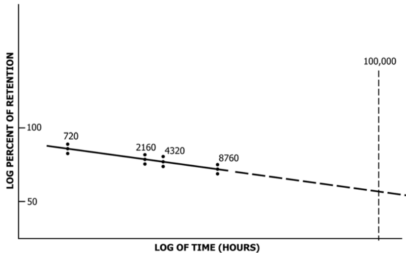
FIG. 3 Chemical Test Property Retention
