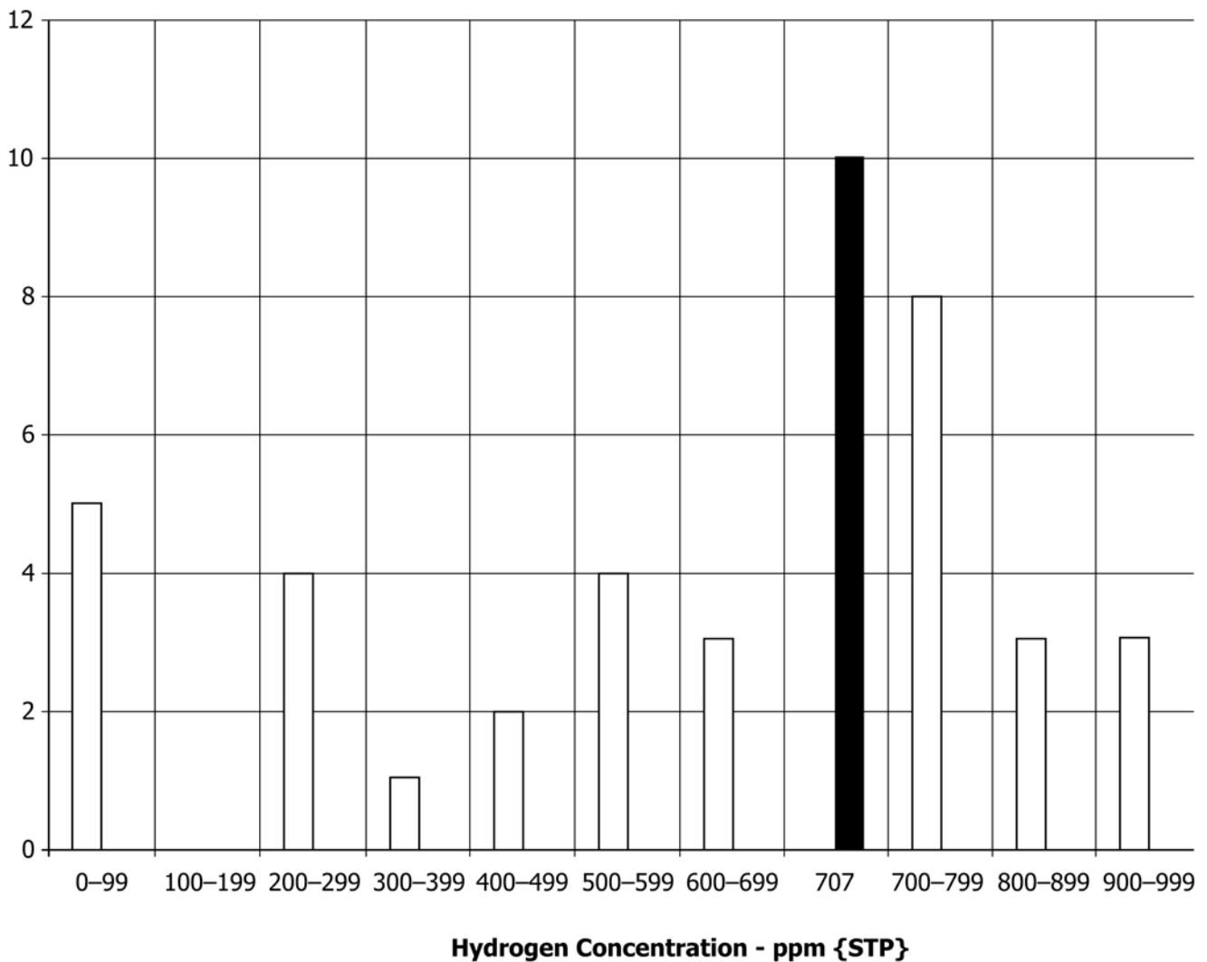
FIG. 6 Distribution of D 3612B Interlaboratory Test Hydrogen Results - Oil Sample - Spiked @ 707 ppm (STP) H2
