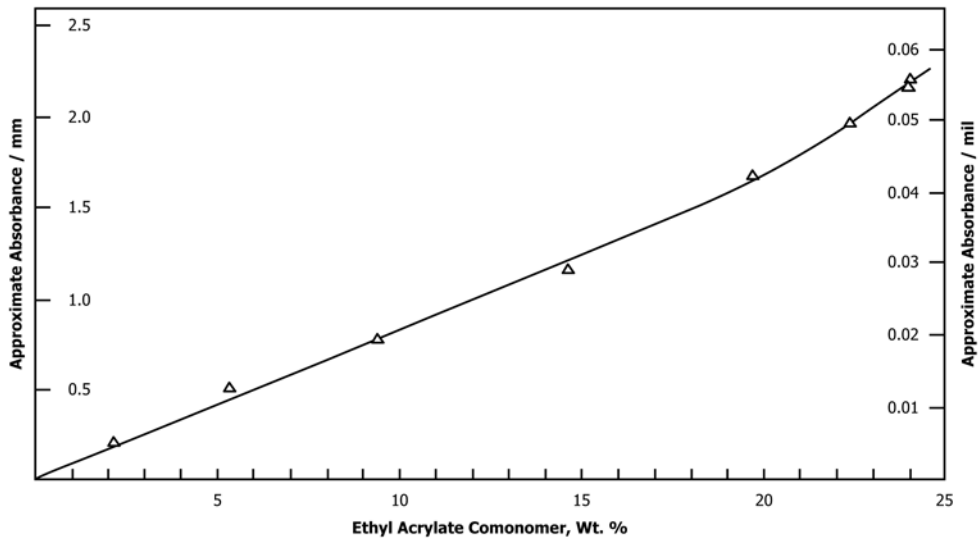
FIG. 2 Example of Typical Calibration Curve for Ethyl Acrylate Comonomer in Ethylene-Ethyl Acrylate Copolymer at 11.6 μm
