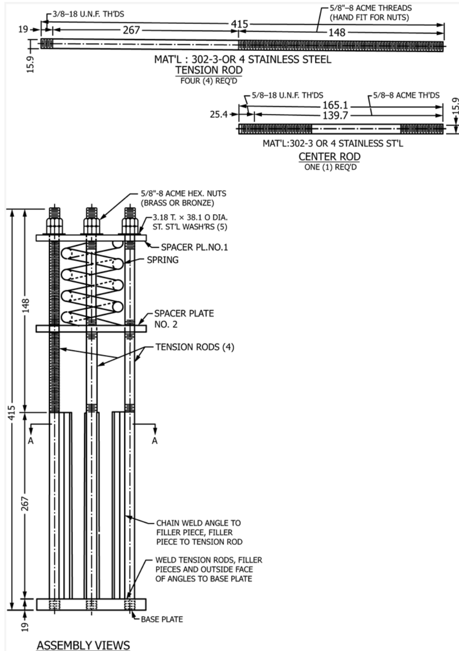
FIG. 2 Optional Compression-Type Creep Tester
