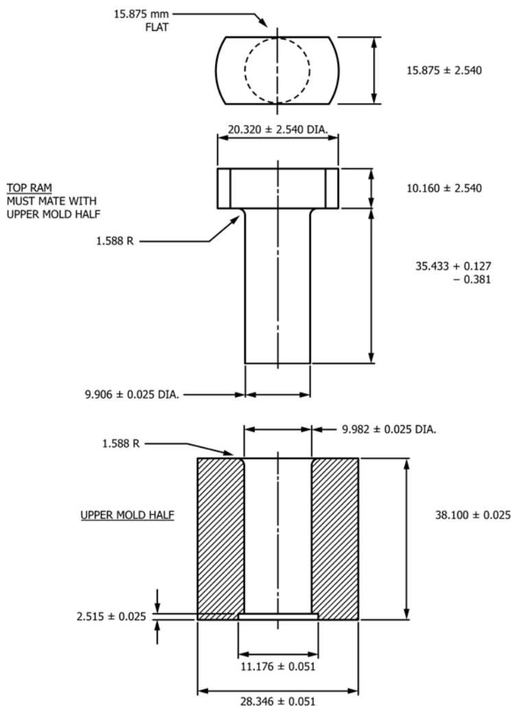
FIG. 4 Upper Half of Mold Assembly for Pressure Molding Asphalt and Pitch into a Specimen Cup
