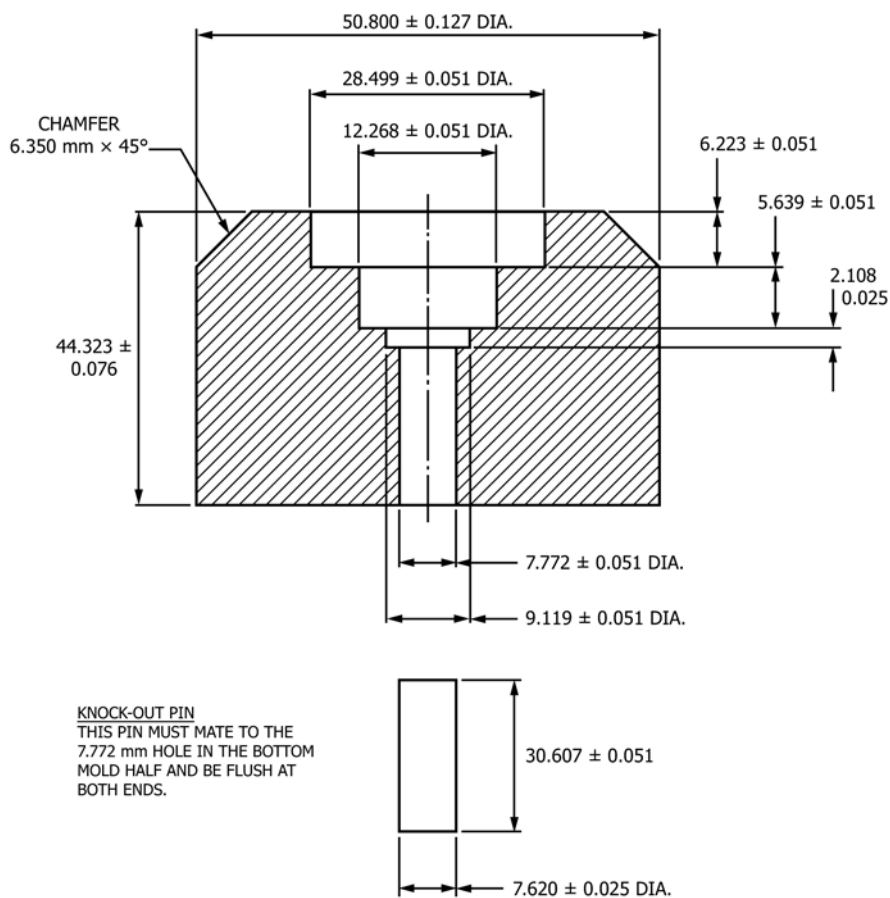
FIG. 5 Lower Half of Mold Assembly for Pressure Molding Asphalt and Pitch into a Specimen Cup
