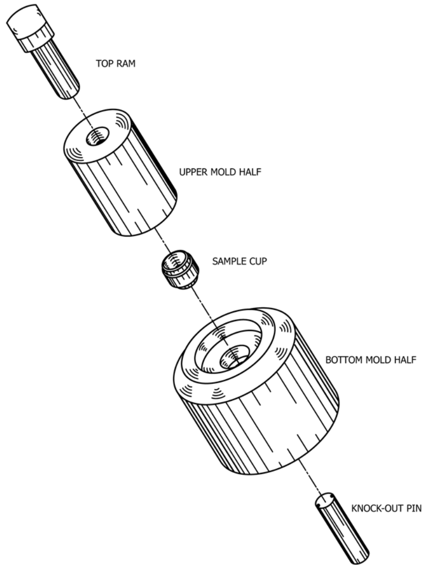
FIG. 6 Assembly of Mold for Pressure Molding Asphalt and Pitch into a Specimen Cup
