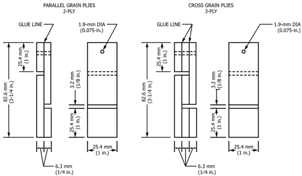
FIG. 3 Test Specimens
