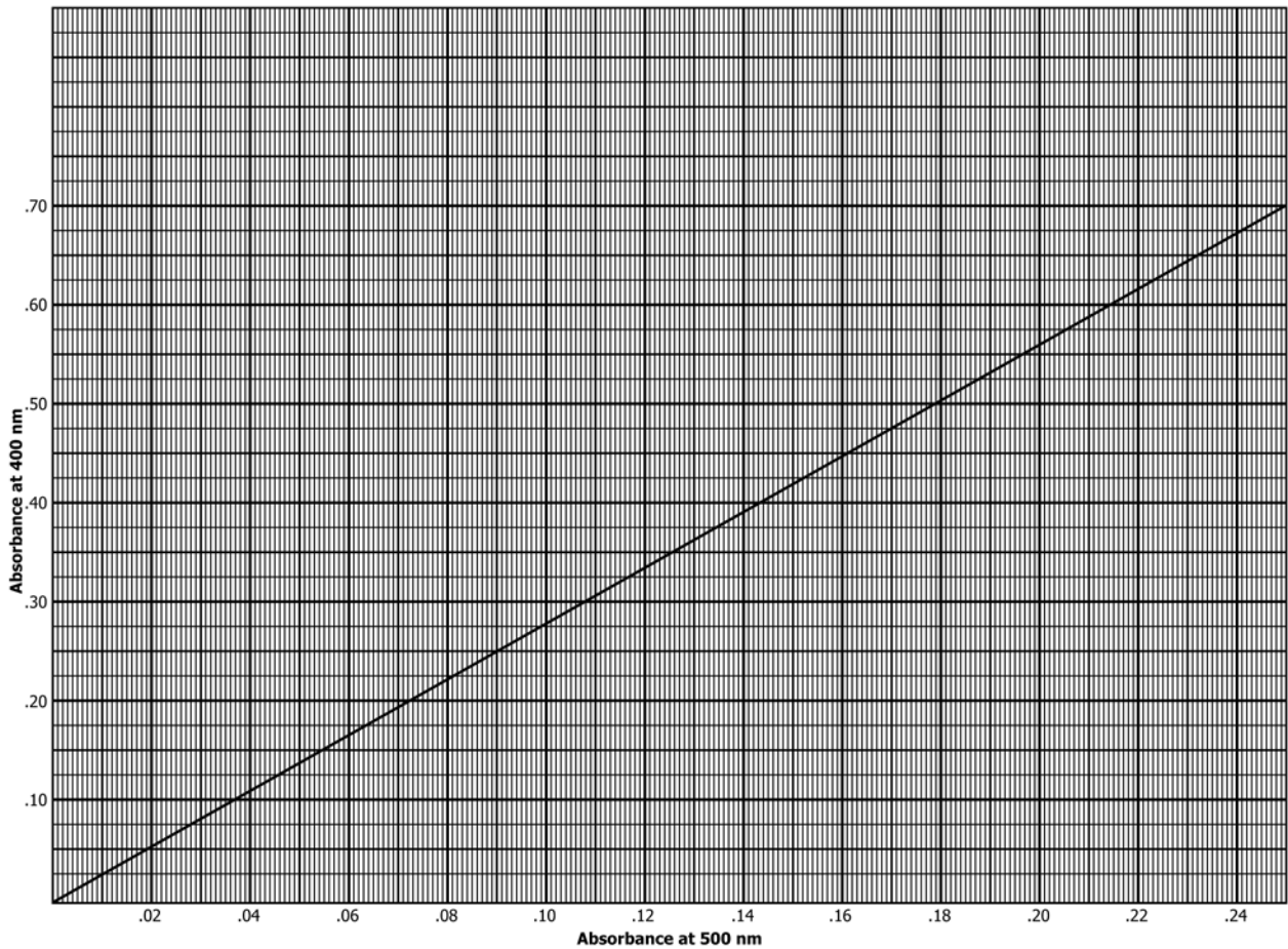
FIG. 1 Correction Graph
