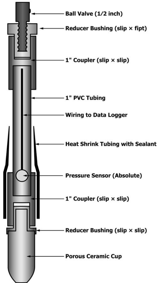
FIG. 5 Portable Tensiometer Design to Be Lowered Down Borehole with Porous Cup in Contact with Geologic Material at Bottom of Well (41)
