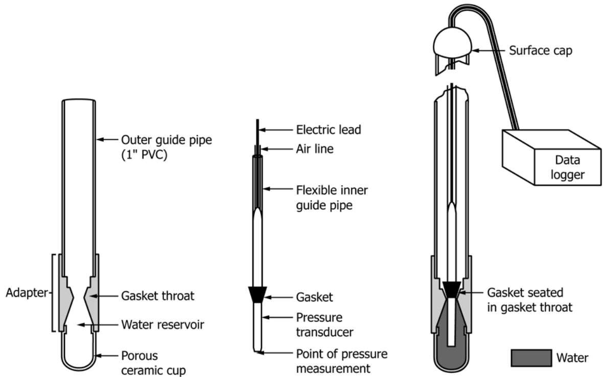
FIG. 4 Advanced Tensiometer (two-piece) Design with Permanently Installed Outer Guide Pipe with Porous Cup Assembly and the Pressure Sensor Apparatus (13)
