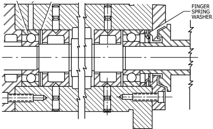
FIG. 1 Test Spindle (Both Bearings Floating)
