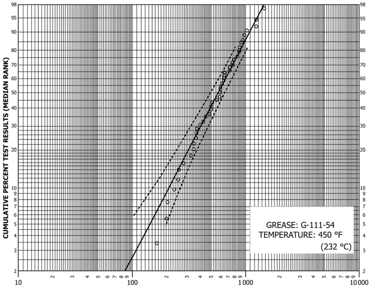
FIG. 4 G-111-54 Grease Life, Hours to Failure
