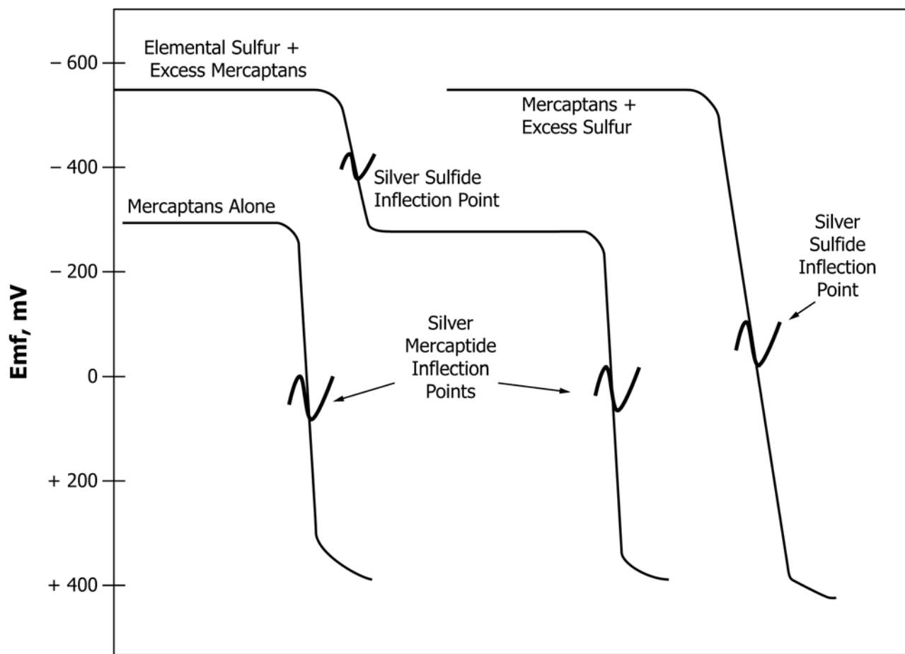
FIG. 1 Illustrative Potentiometric Titration
