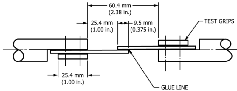
FIG. 1 Test Specimen
