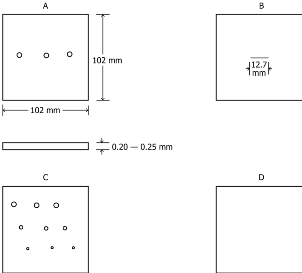
A—3 holes of appropriate diameter B—One 12.7-mm (1/2-in.) slit of appropriate width C—9 holes—3 each 0.254, 0.508, and 0.762 mm (0.010, 0.020, and 0.030 in.) in diameter (bored on a diagonal) so that drainage from one hole will not flow across another hole D—Solid
