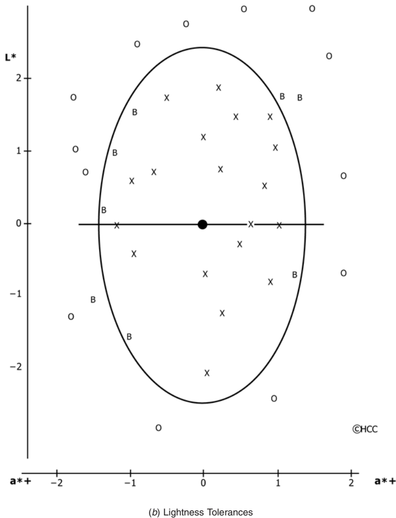
NOTE 1—The standard color is at the 0,0 point and the tolerance ellipses define permissible differences from it. Fig. 2(a) shows chromaticity tolerances in a^* and b^* ; Fig. 3(b) shows lightness tolerances in L^* , with a^* data also shown.
