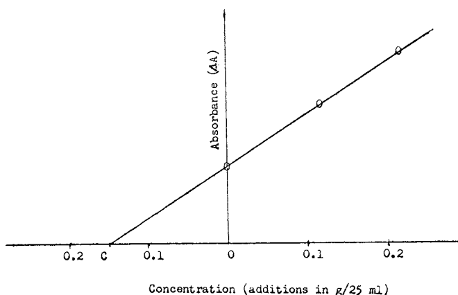
FIG. 1 Plot of ΔA versus Cellulose Nitrate Additions
