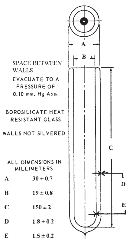
FIG. 1 Specimen Tube
