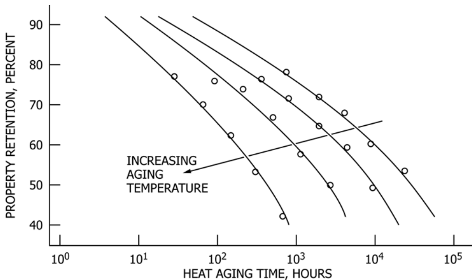
FIG. 1 Heat Aging Curves—Property Retention Versus Aging Time
