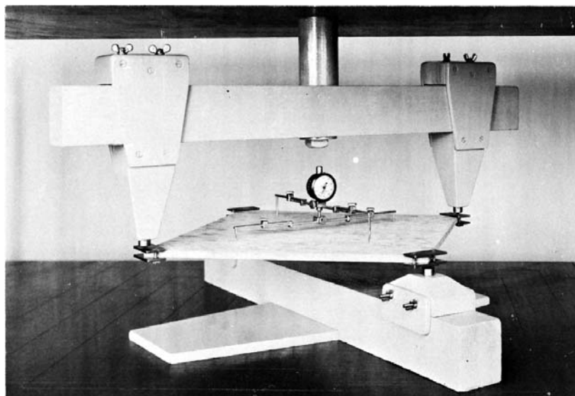
FIG. 1 Shear Modulus Test of Structural Panel Showing Method of Loading and Observing the Deflections Along the Diagonals
