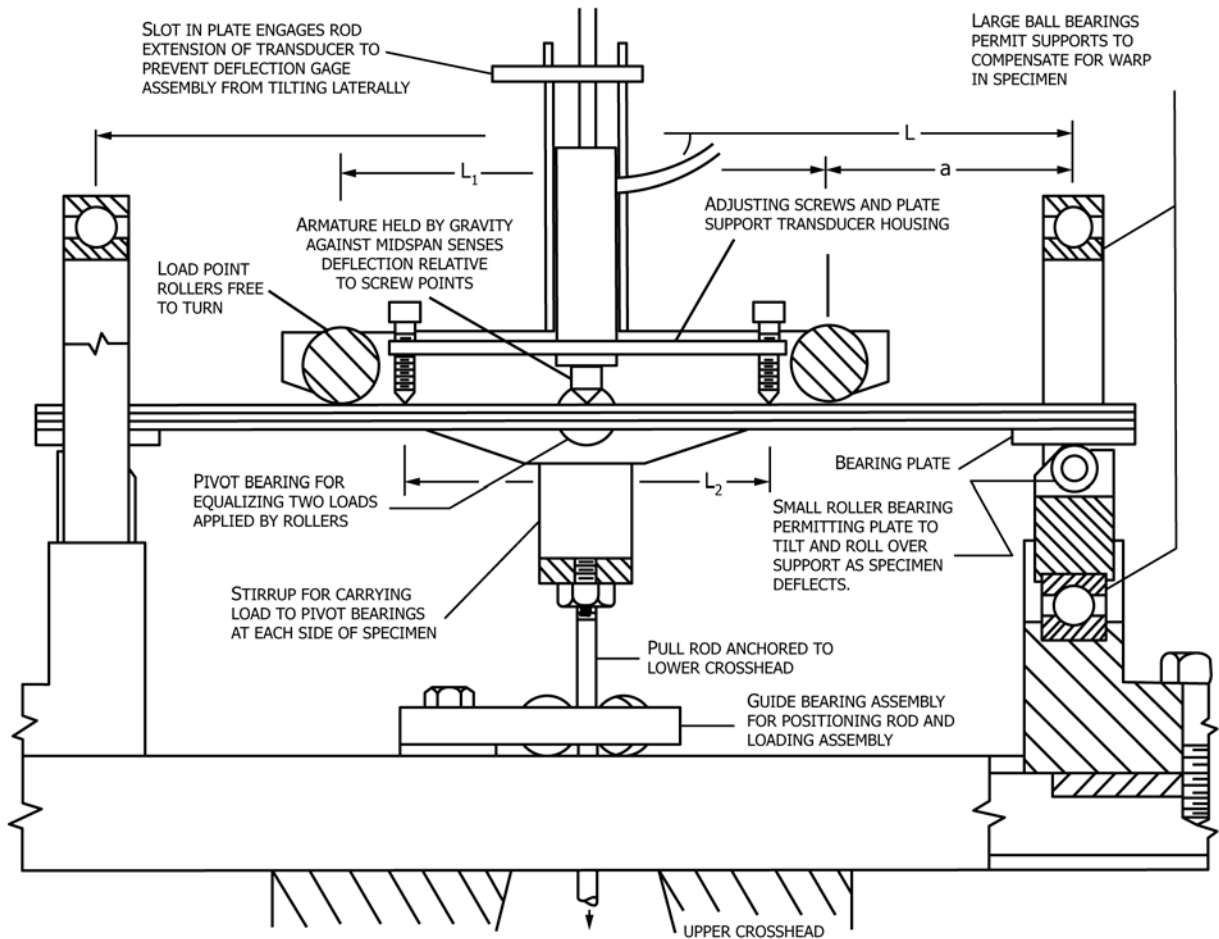
FIG. 6 Two-Point Load Test (Method B)
