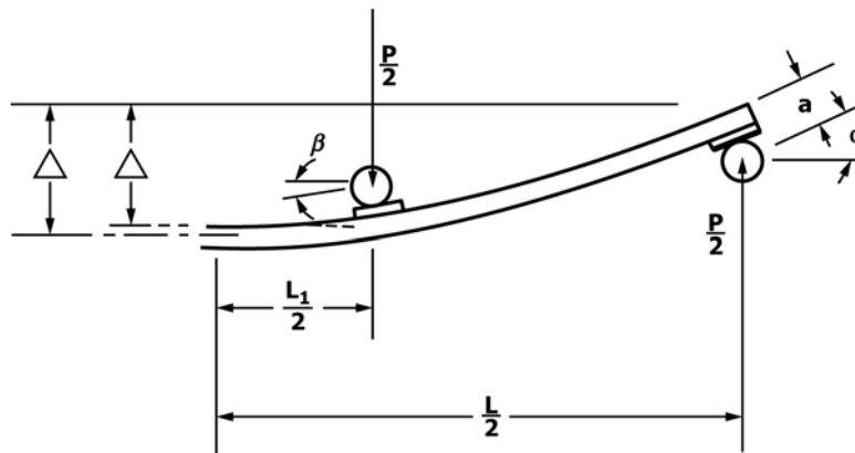
FIG. X1.1 True Moment Calculation in Center-Point Load Test
