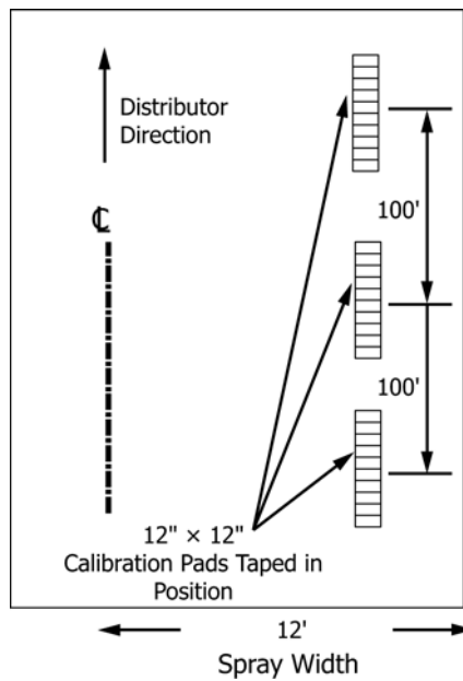
FIG. 3 Position of Pad Assemblies for Longitudinal Rate Determination
