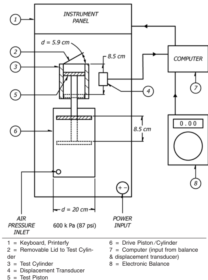
FIG. 1 Compressed Volume Densimeter
