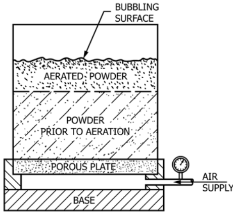
FIG. 1 Aerated Bed
