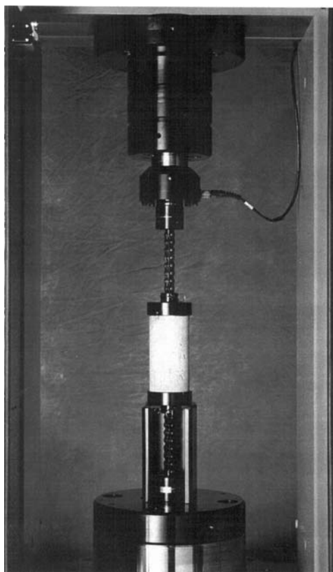
FIG. 1 Direct Tensile-Strength Test Assembly
