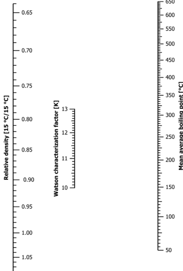
FIG. A8.1 Watson Characterization Factor of Petroleum Fractions
