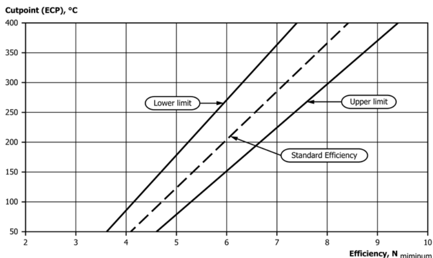
FIG. X2.2 Efficiency Nomograph
