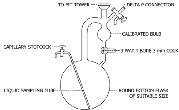
FIG. A1.2 Boiling Rate Timer
