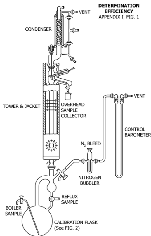
FIG. A1.1 Determination of Efficiency
