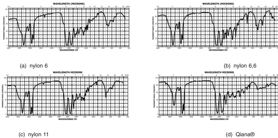
FIG. 13 Infrared Absorption Spectra of Typical Nylon Fibers
