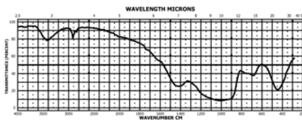
FIG. 10 Infrared Absorption Spectrum of a Typical Glass Fiber
