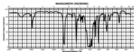
FIG. 16 Infrared Absorption Spectrum of a Typical Polycarbonate Fiber
