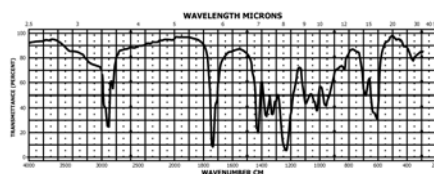
FIG. 23 Infrared Absorption Spectrum of a Typical Vinal Fiber
