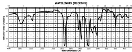
FIG. 14 Infrared Absorption Spectrum of a Typical Nitril Fiber
