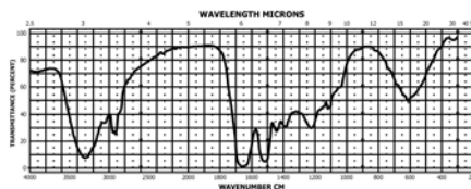
FIG. 25 Infrared Absorption Spectrum of a Typical Wool Fiber
