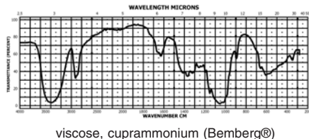
FIG. 18 Infrared Absorption Spectrum of a Typical Rayon Fiber
