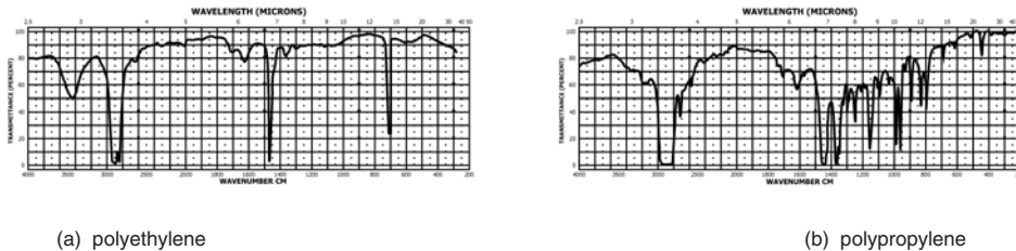
FIG. 15 Infrared Absorption Spectra of Typical Olefin Fibers
