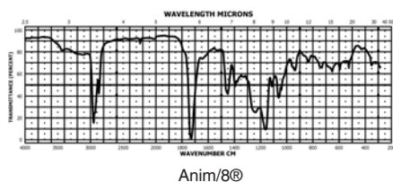
FIG. 5 Infrared Absorption Spectrum of a Typical Anidex Fiber
