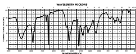
FIG. 3 Infrared Absorption Spectrum of a Typical Acetate Fiber
