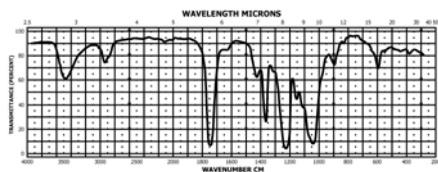
FIG. 3 Infrared Absorption Spectrum of a Typical Acetate Fiber
