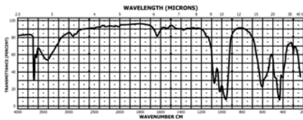
FIG. 7 Infrared Absorption Spectrum of a Typical Asbestos Fiber
