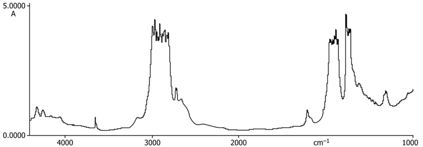
FIG. 6 Example of a FTIR Scan on a Transformer Oil with 0.55 % DBPC
