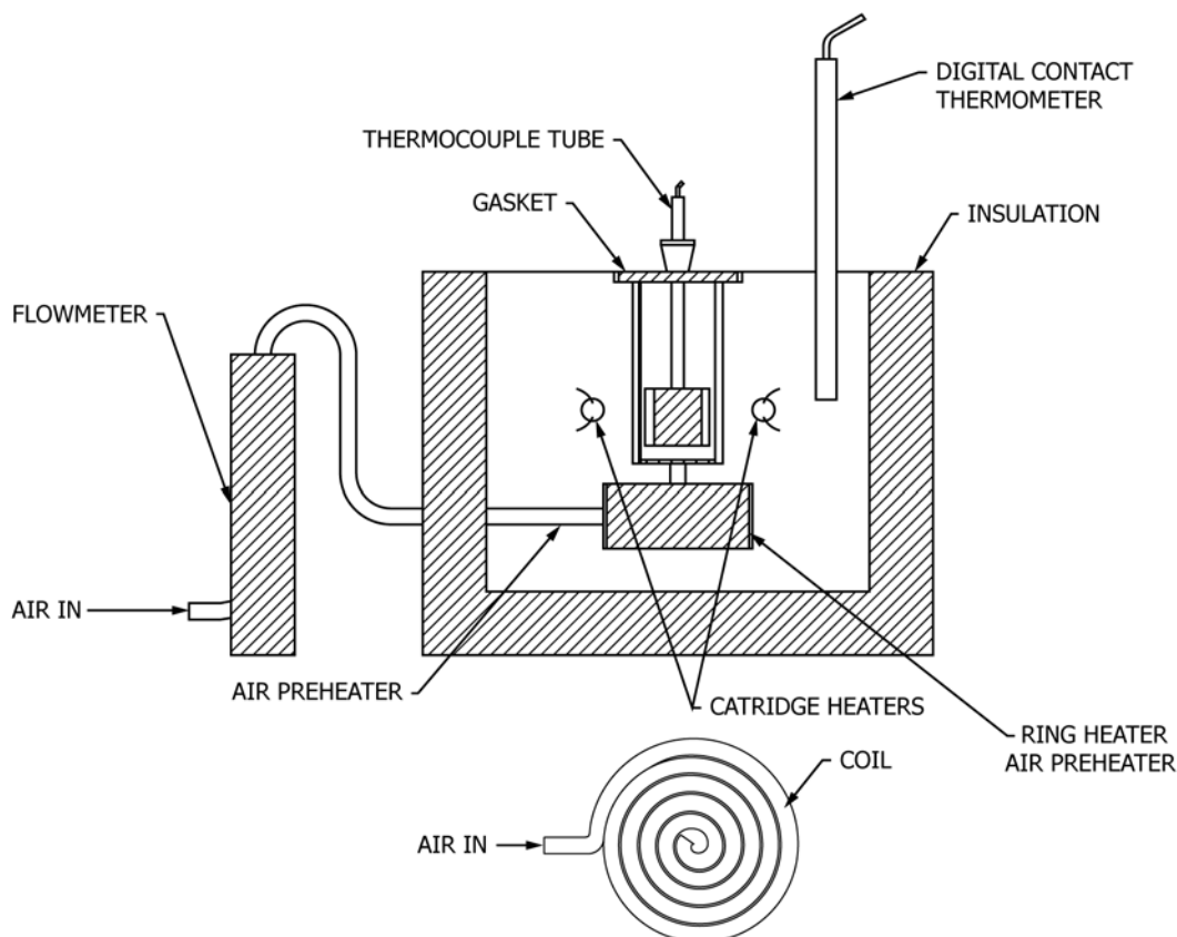
FIG. 4 Aluminum Block Heater
