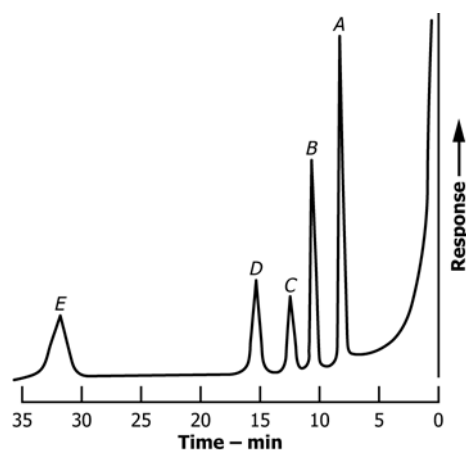
NOTE 1—Analyses were made with 3-m by 3-mm (10-ft by 1/8-in.) stainless steel column coated with 20 % Carbowax-terephthalic acid on 60/80-mesh diatomite, HMDS treated. Column temperature was 210°C, and injection temperature, 250°C. Hydrogen and helium flow rates were each 20 mL/min, at electrometer range 1 and attenuation 1, with chart speed at 305 mm (12 in.)/h, 1-mV full-scale response, and 1-μL sample of approximately 100-mg/L solutions of each phenolic. Peak A is for o -chlorophenol; B, phenol; C, m -cresol; D, 2,4-dichlorophenol; E, p -chlorophenol.
