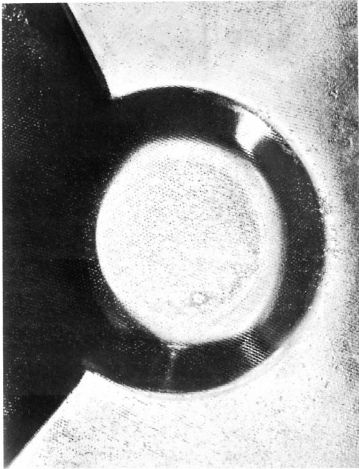
FIG. 12 Porosity
