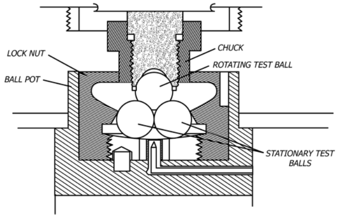
FIG. 2 Falex Corporation (Roxanna) Four-Ball Test Arrangement
