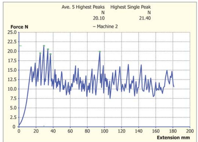
FIG. 3 Typical Tongue Tearing Force-Extension Curves for Individual Specimens (Typical woven cotton fabric)
