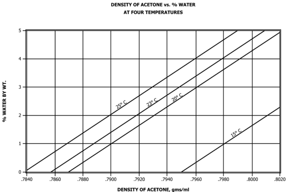
FIG. X1.1 Density of Acetone versus Percent Water at Four Temperatures
