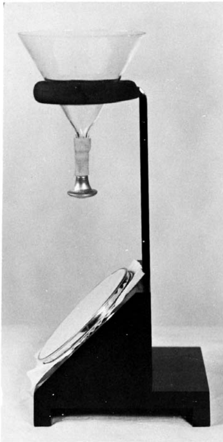
FIG. 1 Spray Tester
