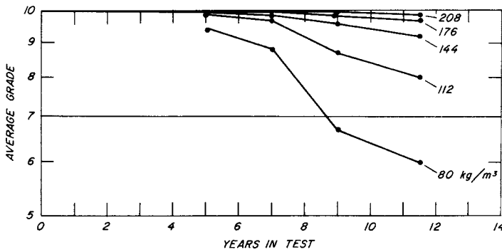
FIG. 3 Example of Depreciation Curves: Low-Residue Creosote 80, 112, 144, 176, and 208 kg/m³
