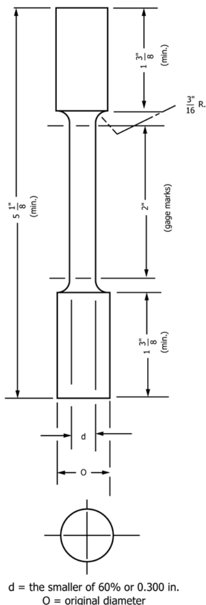
FIG. 1 Turned Dumbbell Specimen for Tensile Testing
