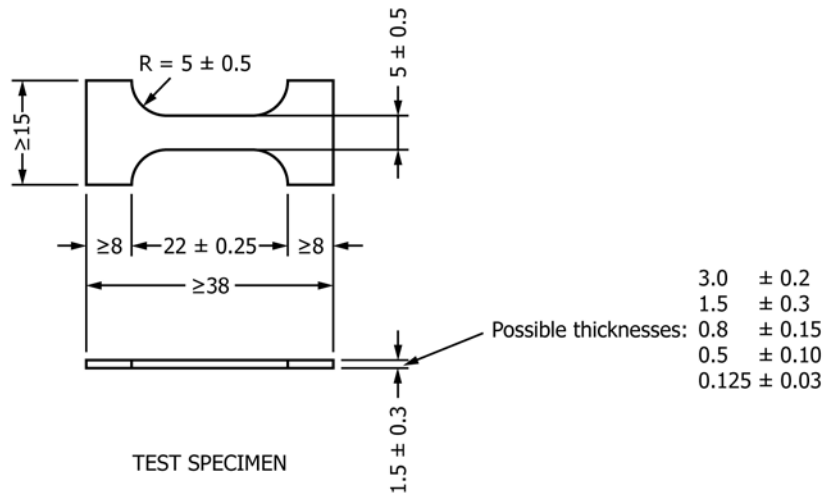
NOTE 1—All dimensions are in millimetres. FIG. 1 Microtensile Die and Test Specimen
